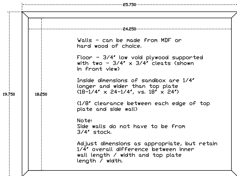
Sandbox - Top View (See front view for cleat detail on floor)
