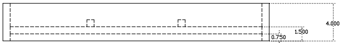
Sandbox - Front View Showing floor with 2 - (3/4" x 3/4") support cleats (footers with T-nuts not shown - see note at right)
